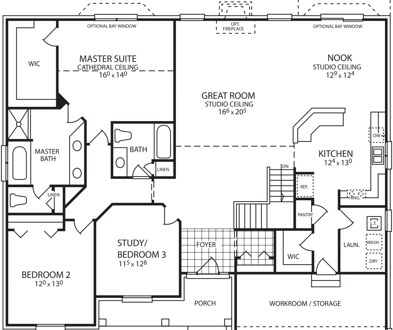
FLOOR PLAN
